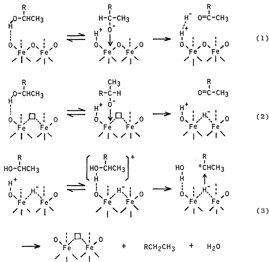
Scheme. Reaction scheme over Fe 2 O 3 and reduced Fe 2 O 3 .
